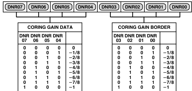
Figure 78. DNR Register 0 in DNR Mode
