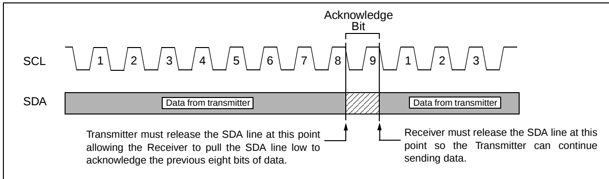
FIGURE 6-4: ACKNOWLEDGE TIMING
