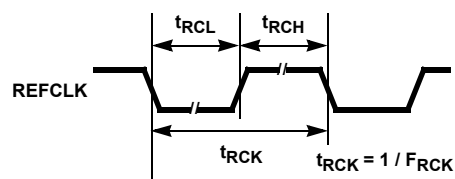
FIGURE 25. REFCLK TIMING
