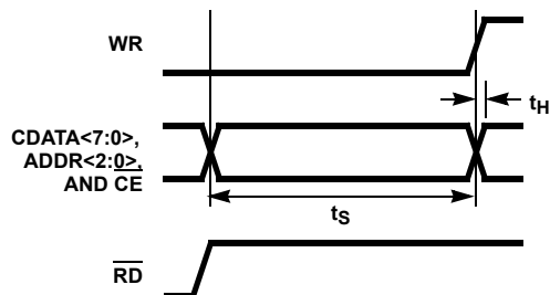
FIGURE 24. TIMING RELATIVE TO WR, LOADING SEQUENCE
