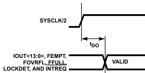
FIGURE 27. SYSCLK/2 RELATIVE TIMING
