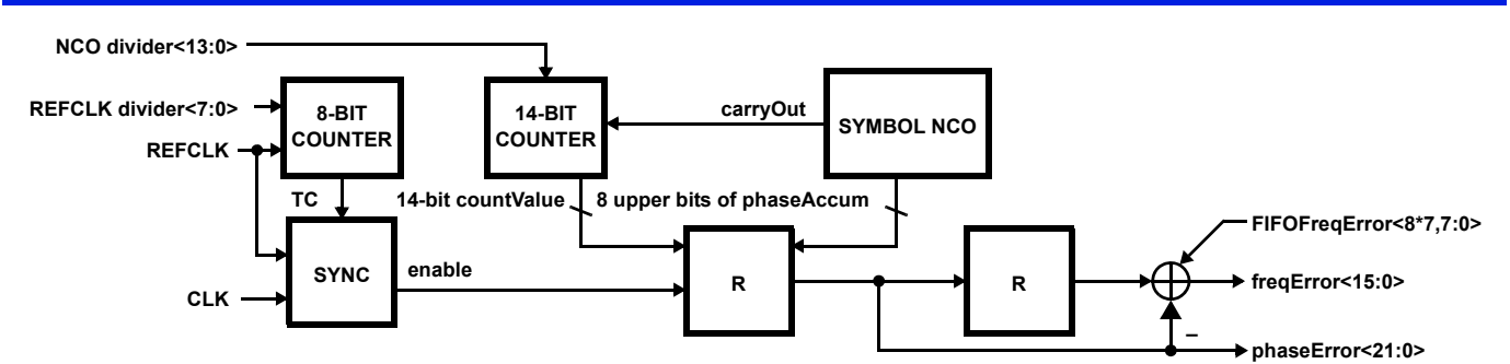
FIGURE 2. PHASE/FREQUENCY ERROR DETECTOR
