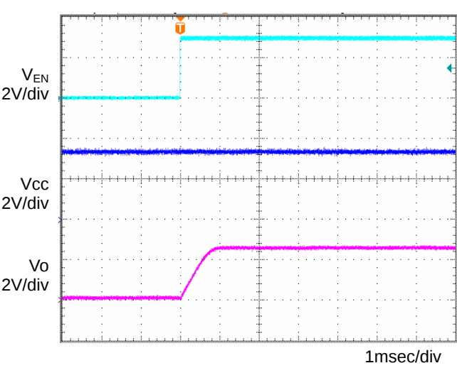
Fig.17 Input sequence 2 \text{Co}=1\mu\text{F} , T_a=105^{\circ}\text{C}
