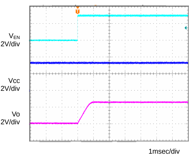
Fig.15 Input sequence 2 \text{Co}=1\mu\text{F} , T_a=-40^{\circ}\text{C}
