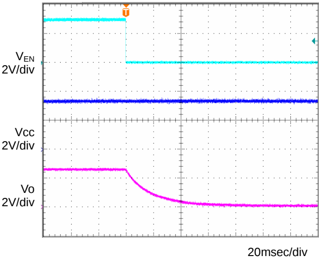
Fig.18 OFF sequence 2 \text{Co}=1\mu\text{F} , T_a=-40^{\circ}\text{C}
