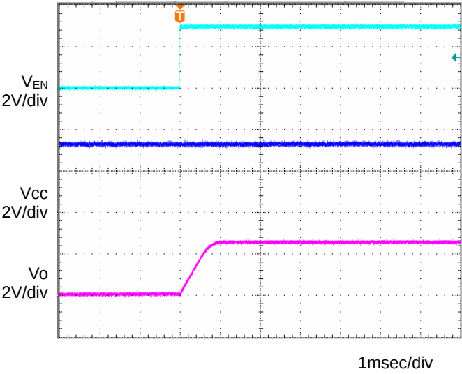
Fig.16 Input sequence 2 \text{Co}=1\mu\text{F} , T_a=25^{\circ}\text{C}
