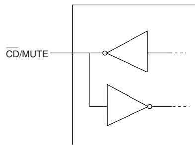
Figure 3-5: \overline{CD/MUTE} Circuit
