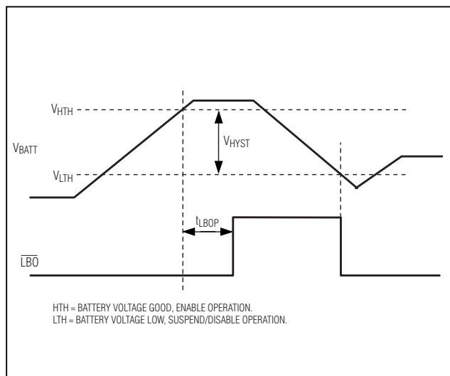
Figure 8. Hysteresis
