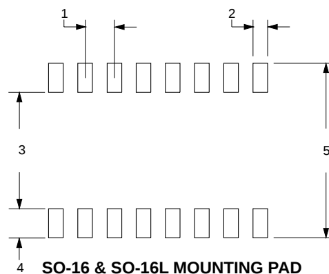
SO-16 & SO-16L MOUNTING PAD
