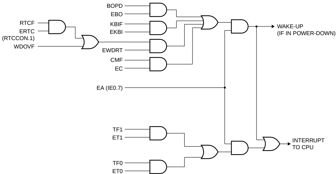
Fig 16. Interrupt sources, interrupt enables, and power-down wake-up sources (P89LPC902).
