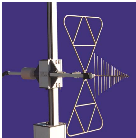
The TDK HLP-3003C Hybrid Log Periodic antenna offers unequalled performance over the ultra wide frequency range of 30 MHz to 3 GHz and an efficient, compact design.
