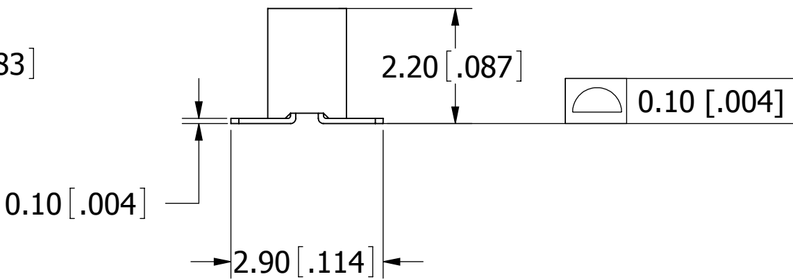
RECOMMENDED PCB LAYOUT SFM210-LP_E-S_-SD-BK
