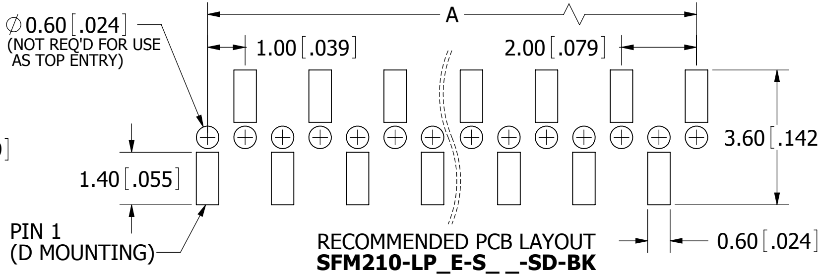
RECOMMENDED PCB LAYOUT SFM210-LP_E-S_-SC-BK
