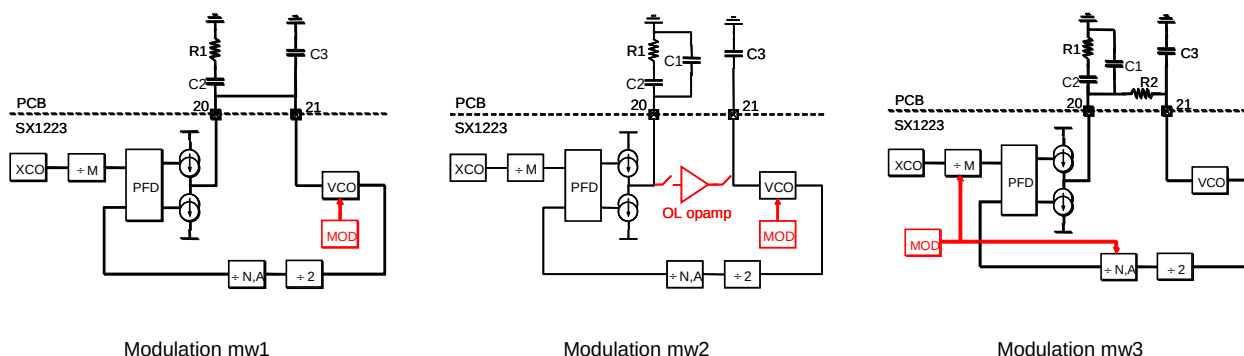
Figure 4: Modulation modes
