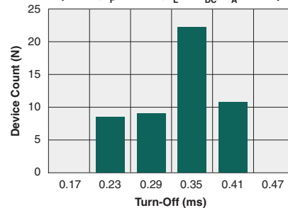
Typical Turn-Off Time ( N=50 , I_F=20\text{mA} , I_L=1A_{DC} , T_A=25^\circ\text{C} )
