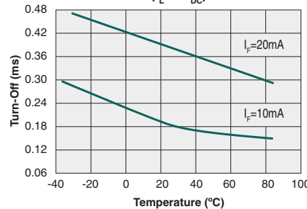
Typical Turn-Off vs. Temperature ( I_L=1A_{DC} )
