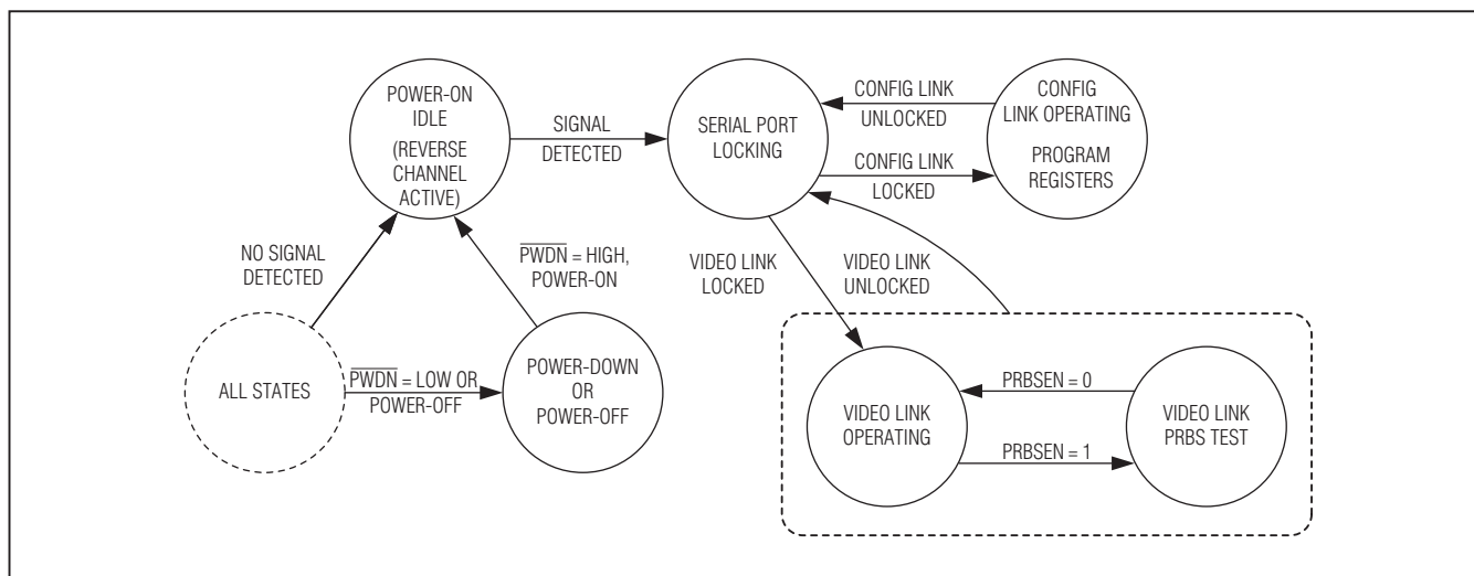
Figure 33. Deserializer State Diagram, CDS = High (Camera Application)
