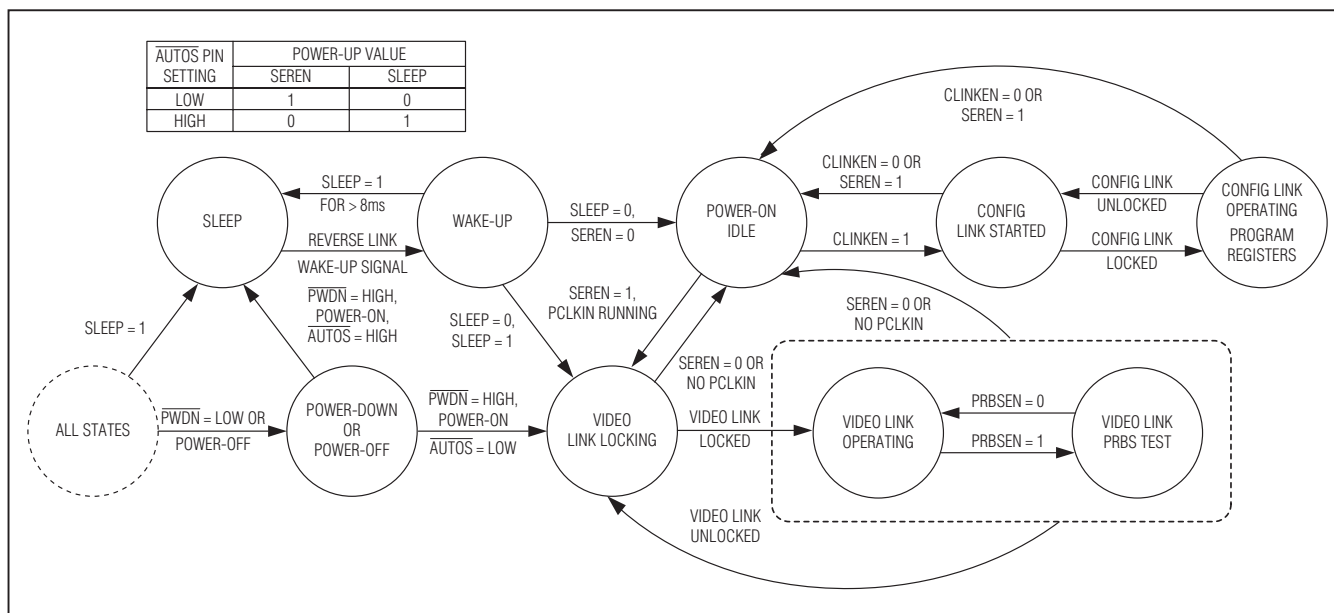
Figure 32. Serializer State Diagram, CDS = High (Camera Application)
