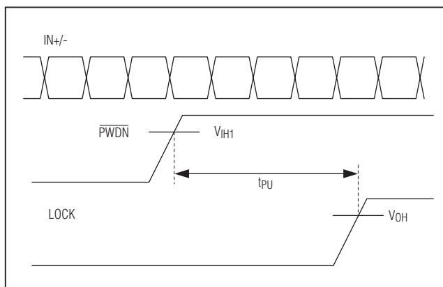
Figure 20. Deserializer Power-Up Delay
