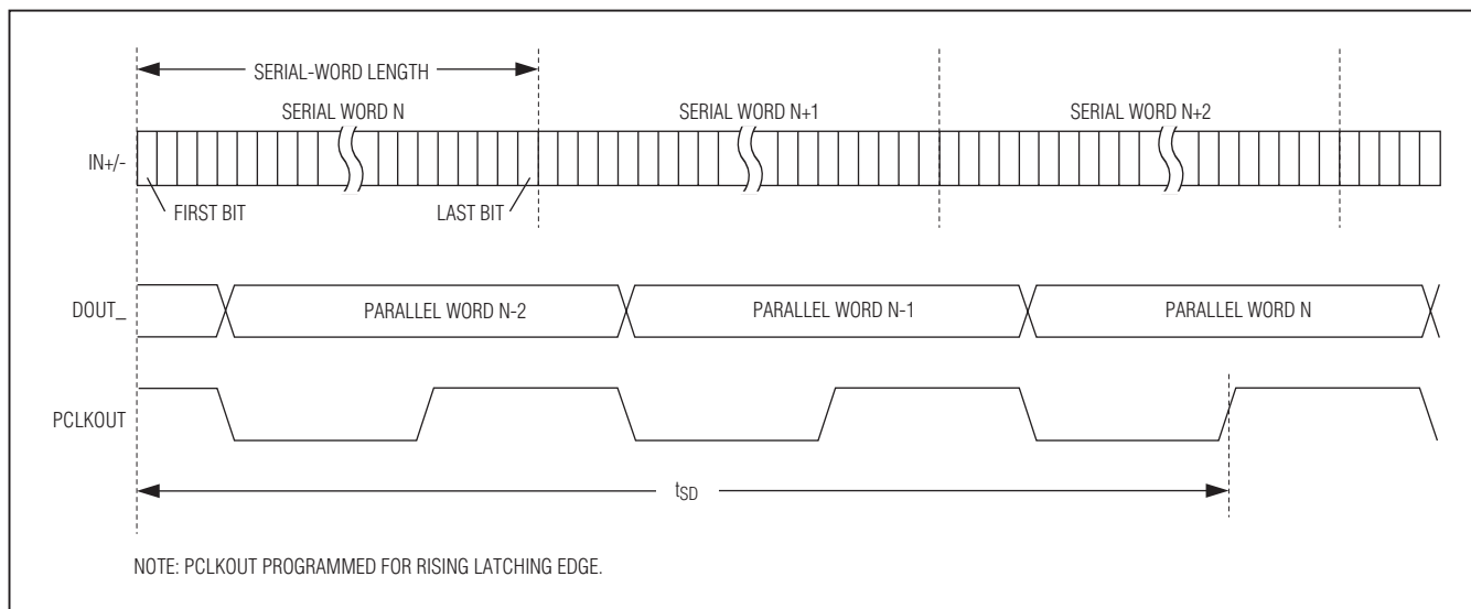
Figure 18. Deserializer Delay
