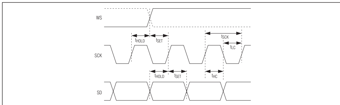
Figure 12. Input I²S Timing Parameters
