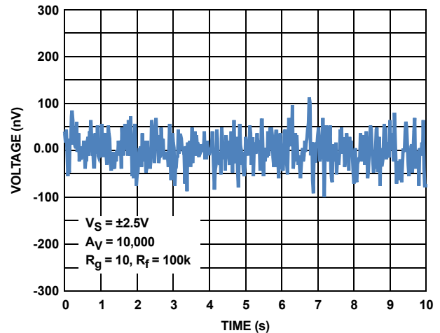
FIGURE 22. INPUT NOISE VOLTAGE 0.1Hz TO 10Hz
