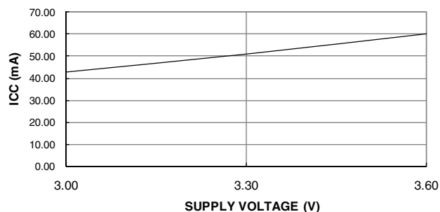
ATMEL ATF22LV10C SUPPLY CURRENT VS. SUPPLY VOLTAGE ( T_A = 25^\circ\text{C} )
