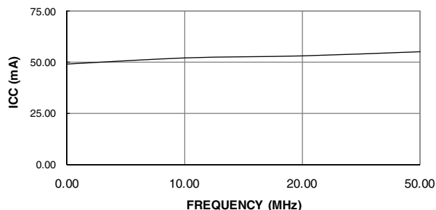
ATMEL ATF22LV10C SUPPLY CURRENT VS. INPUT FREQUENCY ( V_{CC} = 3.3\text{V}, T_A = 25^\circ\text{C} )
