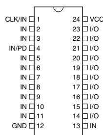
Figure 1-4. DIP/SOIC
