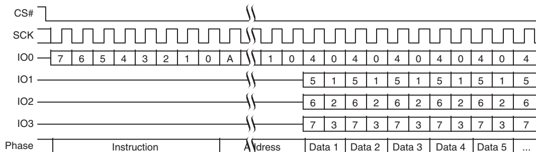
Figure 10.38 Quad Page Program Command Sequence
