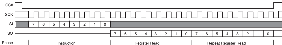
Figure 10.55 PPB Lock Register Read Command Sequence
