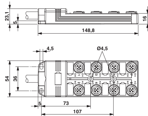
Dimensioned drawing
