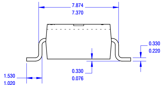
END VIEW
