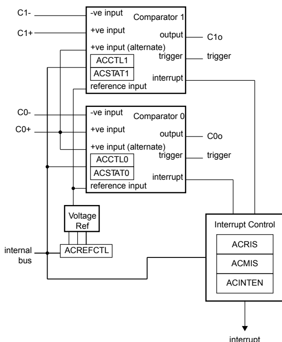
Figure 13-1. Analog Comparator Module Block Diagram
