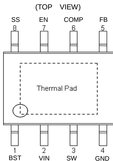
Figure 2. Pin Configuration
