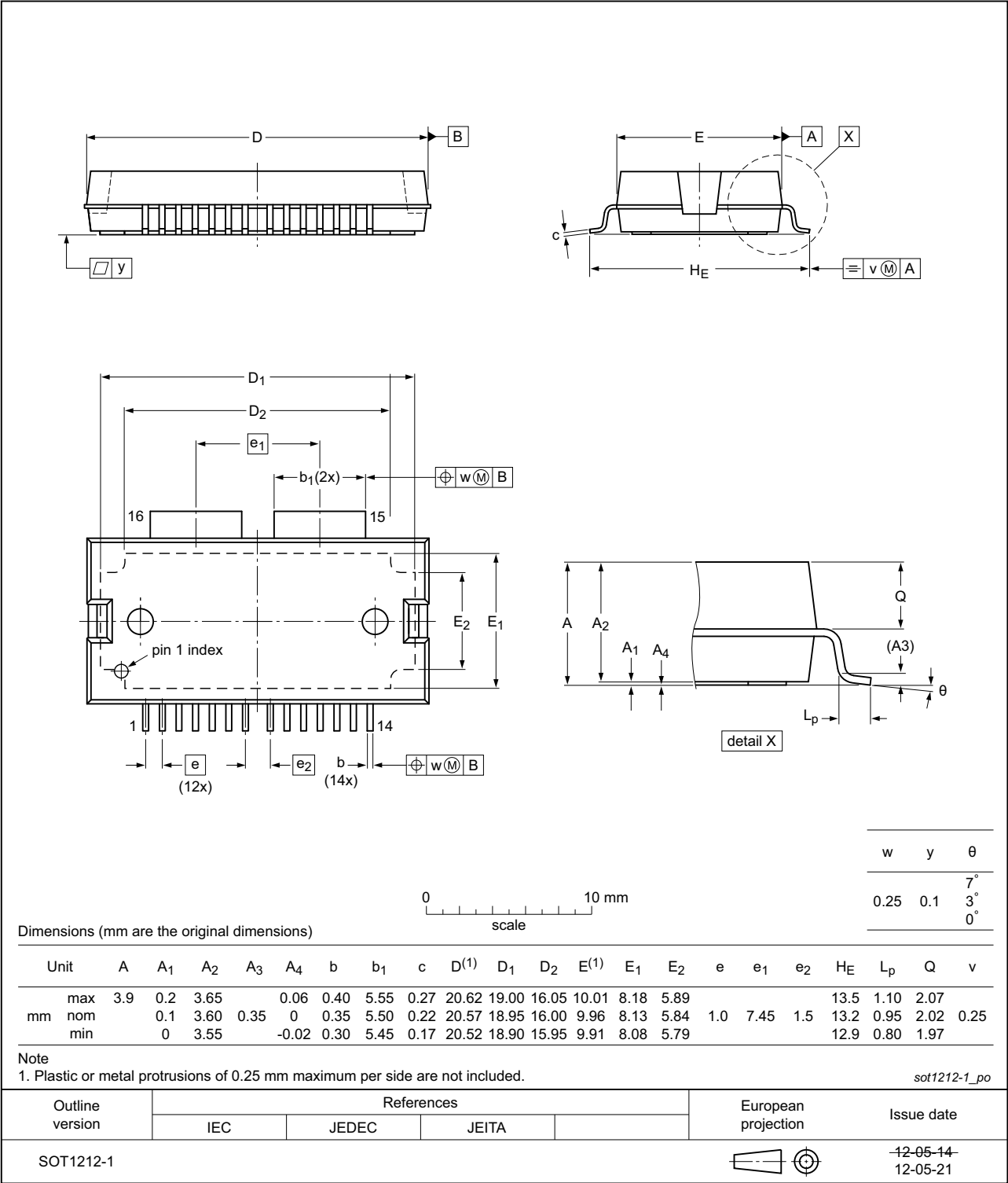
Fig 22. Package outline SOT1212-1 (HSOP16)
