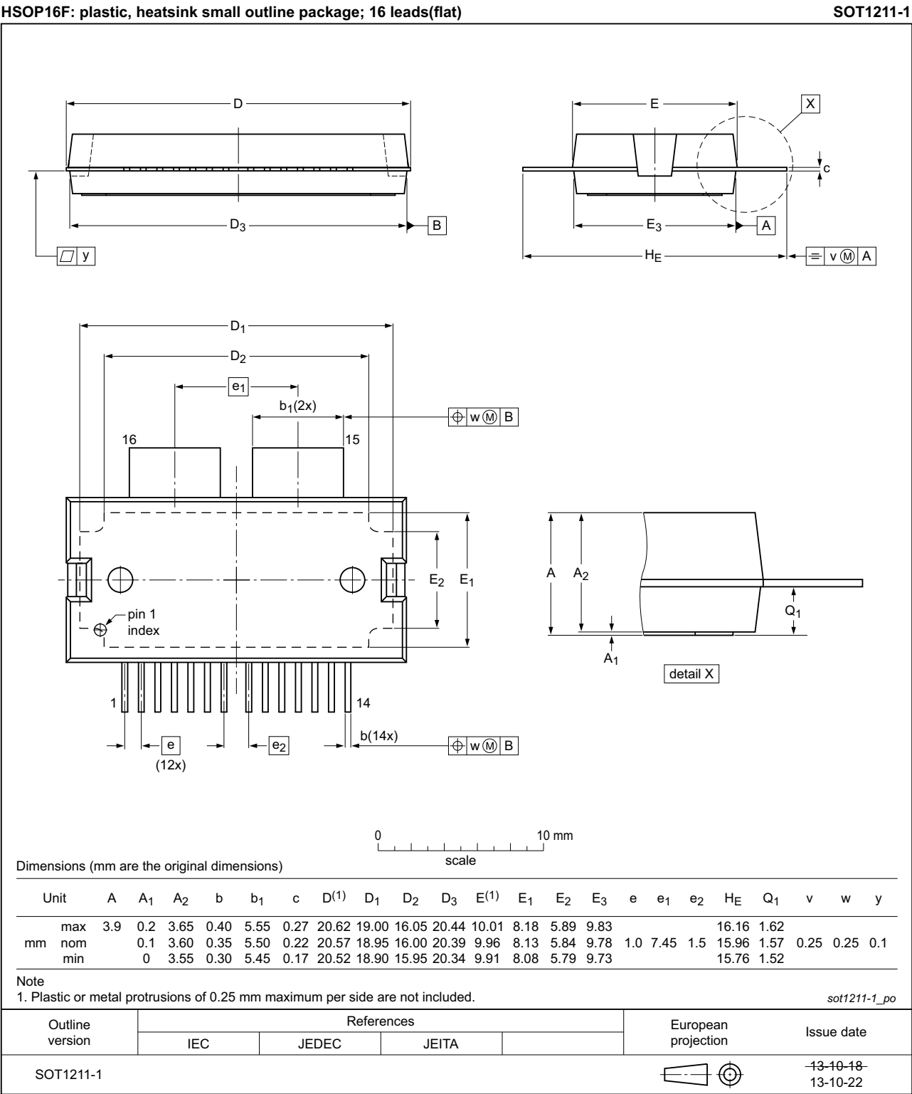
Fig 21. Package outline SOT1211-1 (HSOP16F)
