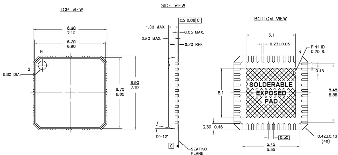
Figure 19. 48-Lead (7x7 mm) QFN (Punched)
