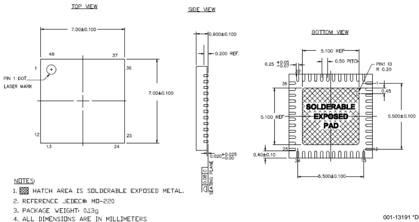
Figure 20. 48-Lead (7x7x1.0 mm) QFN (Sawn)
