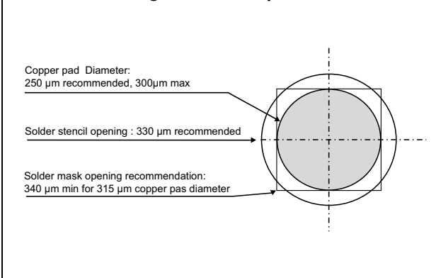
Figure 14. Footprint
