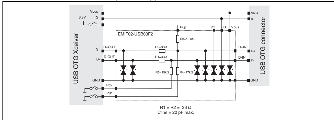
Figure 9. Application schematic
