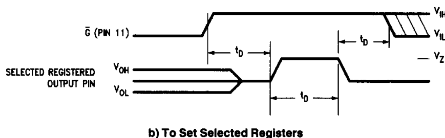
FIGURE 2. Series-D Register Preload Waveforms
