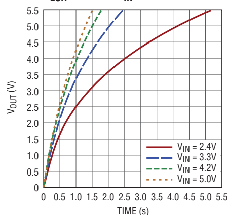
V_{OUT} vs Charge Time, C_{OUT} = 1\text{F} , R_{ESR} = 20\text{m}\Omega , I_{IN} = 3.0\text{A}
