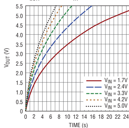
V_{OUT} vs Charge Time, C_{OUT} = 1\text{F} , R_{ESR} = 20\text{m}\Omega , I_{IN} = 0.5\text{A}
