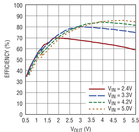
Efficiency vs V_{OUT} (2.0A I_{IN} )
