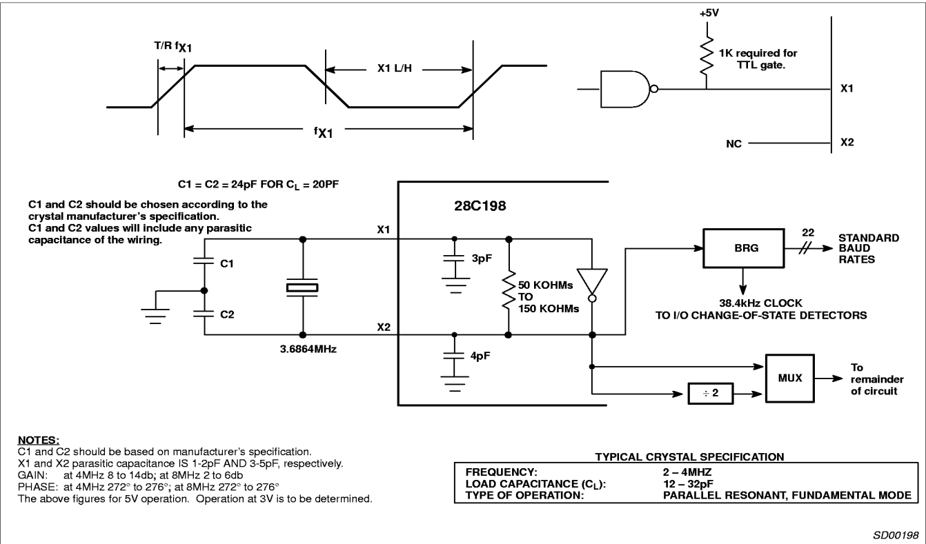
Figure 7. X1/X2 Communication Crystal Clock
