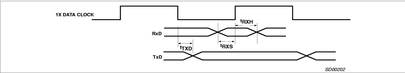
Figure 11. Transmitter and Receiver Timing
