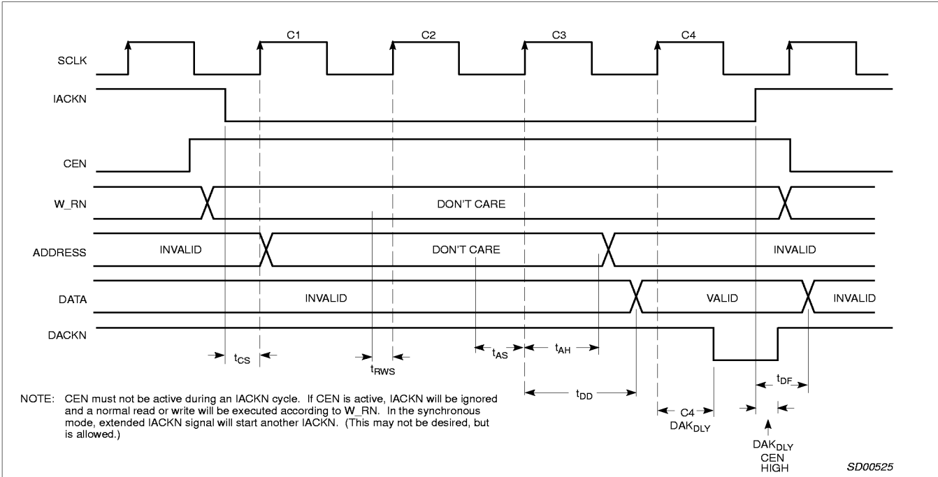
Figure 6. Basic IACKN Cycle, ASYNC/SYNC
