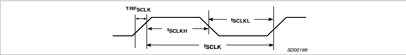
Figure 8. SCLK Timing
