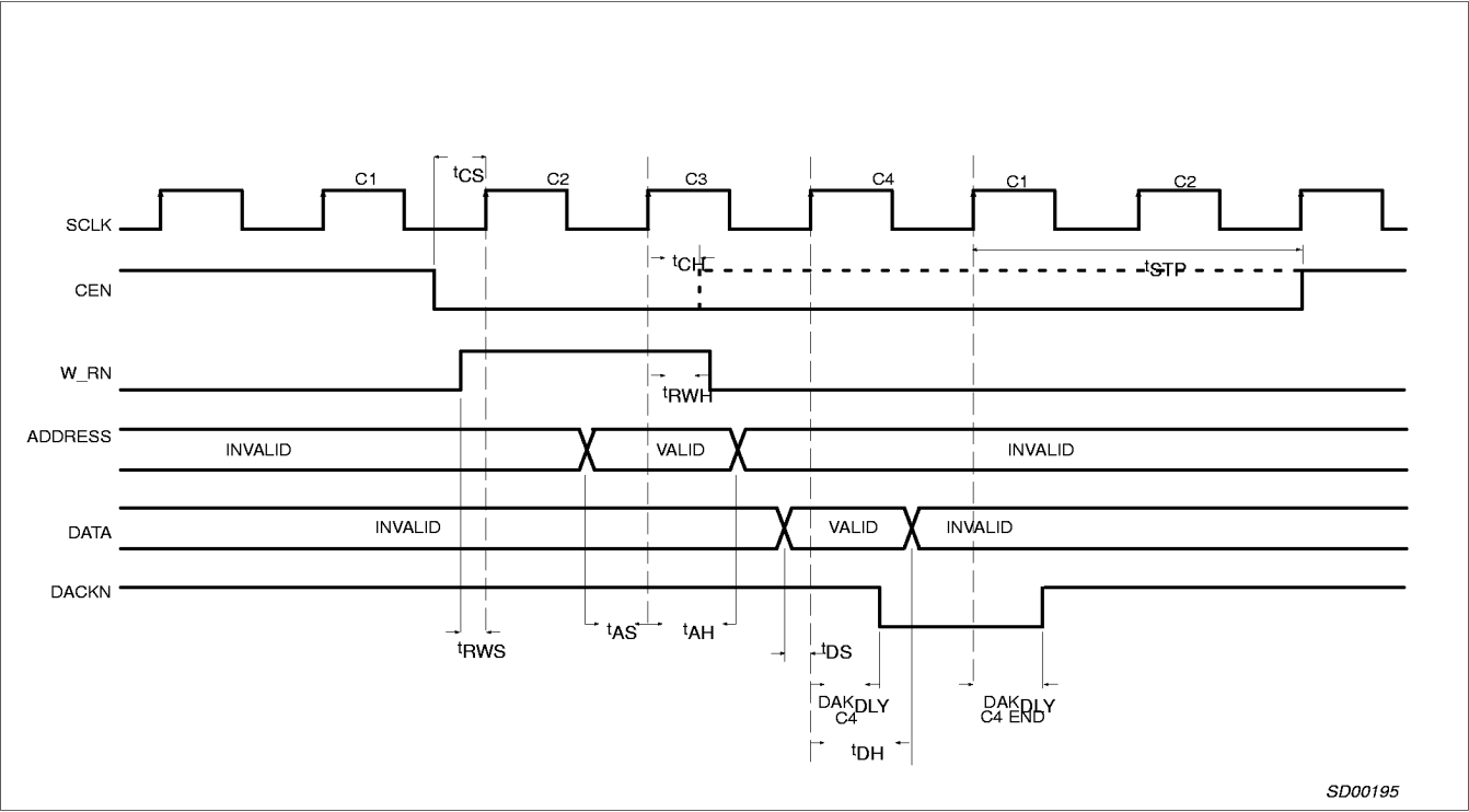
Figure 3. Basic Write Cycle, SYNC
