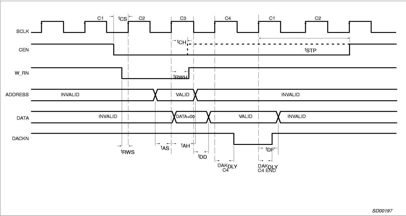
Figure 5. Basic Read Cycle, SYNC
