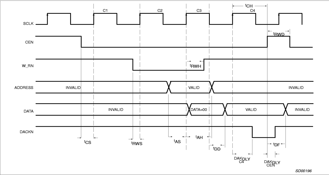
Figure 4. Basic Read Cycle, ASYNC
