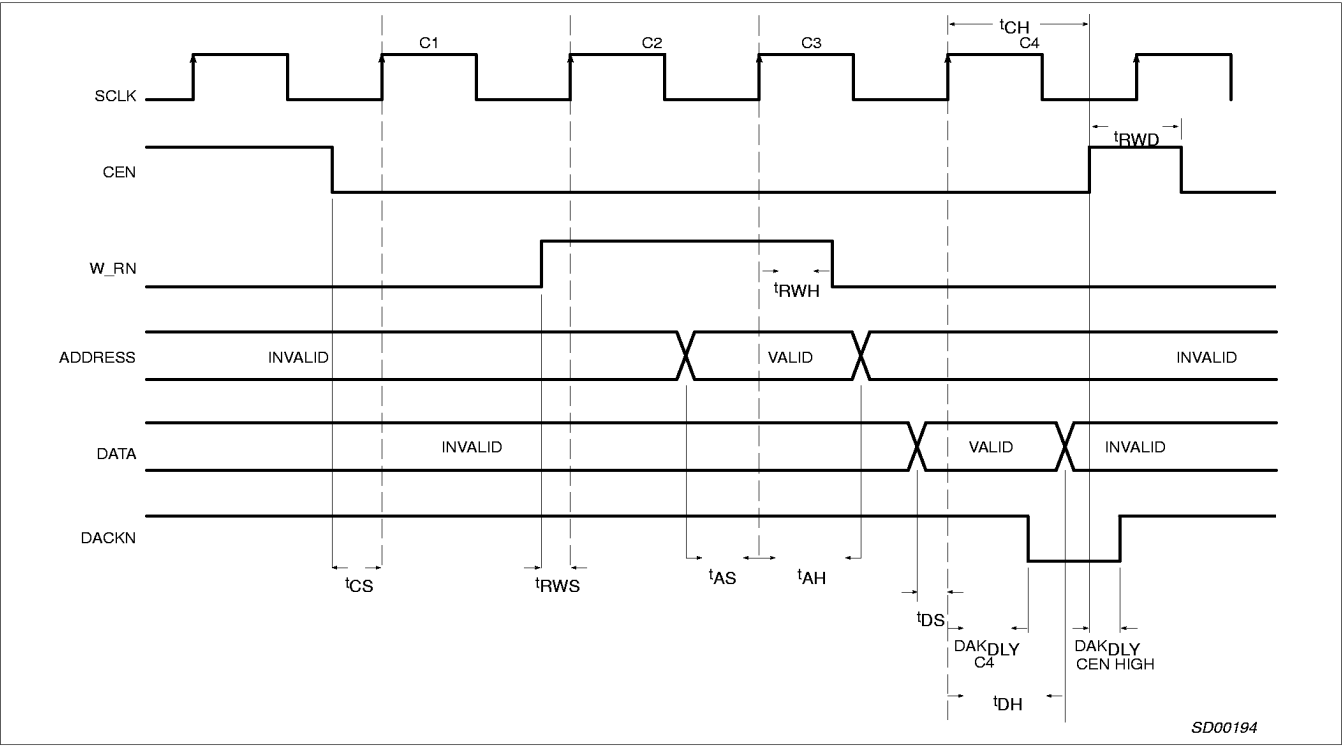
Figure 2. Basic Write Cycle, ASYNC
