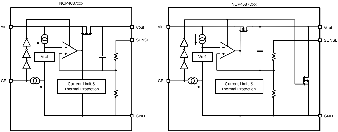
Figure 2. Simplified Schematic Block Diagram
