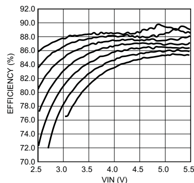
L = 10\text{ }\mu\text{H} 20 mA/String f_{SW} = 1\text{ MHz} Top To Bottom: 2×4, 2×5, 2×6, 2×7, 2×8, 2×9, 2×10 (LEDs)
