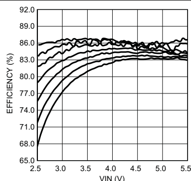
L = 22\text{ }\mu\text{H} 20 mA/String f_{SW} = 1\text{ MHz} Top To Bottom: 1×4, 1×5, 1×6, 1×7, 1×8, 1×9, 1×10 (LEDs)
