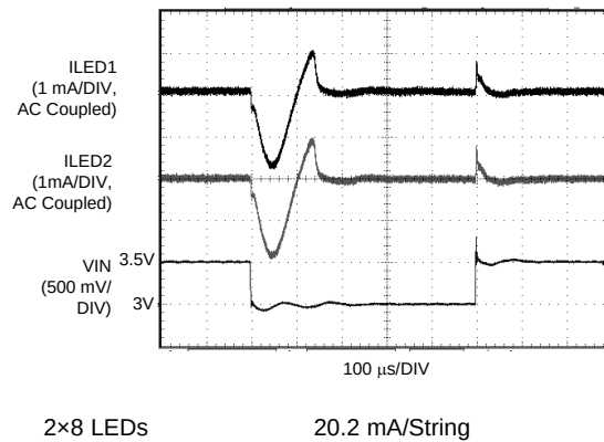
Figure 21. Line Step Response (see Typical Application Circuit )
