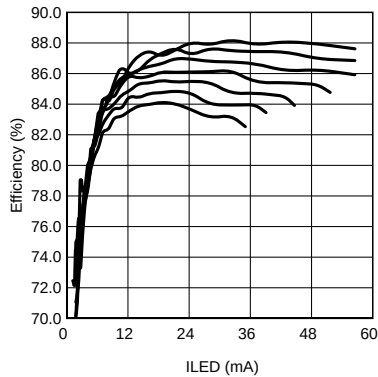
L = 10\text{ }\mu\text{H} V_{IN} = 3.6\text{ V} f_{SW} = 500\text{ kHz} Top To Bottom: 2×4, 2×5, 2×6, 2×7, 2×8, 2×9, 2×10 (LEDs)
