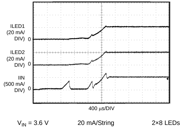
Figure 19. Start-Up Response
