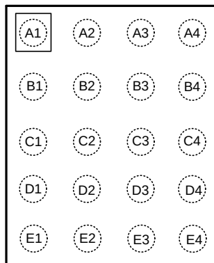
Pin Functions
