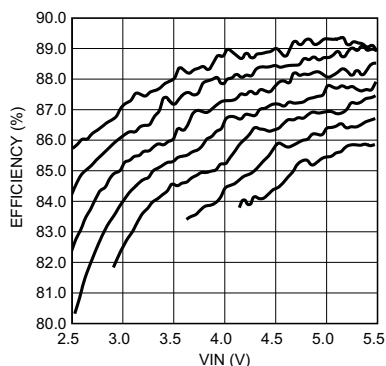
L = 10\text{ }\mu\text{H} 20 mA/String f_{SW} = 500\text{ kHz} Top To Bottom: 2×4, 2×5, 2×6, 2×7, 2×8, 2×9 (LEDs)
