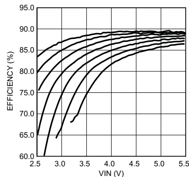
L = 22\text{ }\mu\text{H} 20 mA/String f_{SW} = 1\text{ MHz} Top To Bottom: 2×4, 2×5, 2×6, 2×7, 2×8, 2×9, 2×10 (LEDs)
