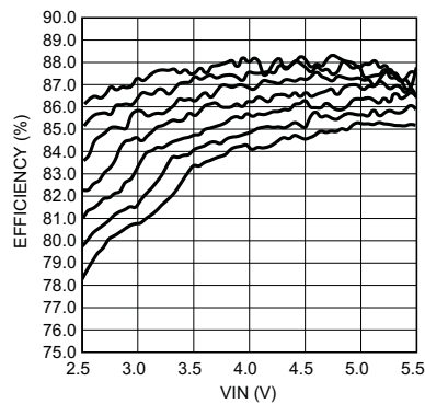
Figure 44. Efficiency vs V_{IN} , Single String
