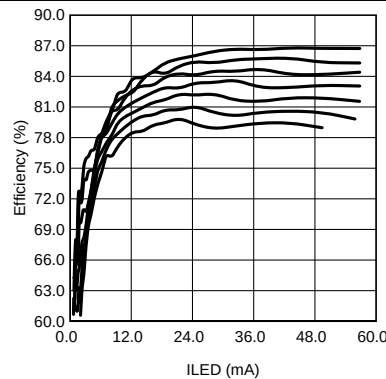
L = 4.7\text{ }\mu\text{H} V_{IN} = 3.6\text{ V} f_{SW} = 1\text{ MHz} Top To Bottom: 2×4, 2×5, 2×6, 2×7, 2×8, 2×9, 2×10 (LEDs)
