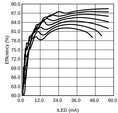
L = 10\text{ }\mu\text{H} V_{IN} = 3.6\text{ V} f_{SW} = 1\text{ MHz} Top To Bottom: 2×4, 2×5, 2×6, 2×7, 2×8, 2×9, 2×10 (LEDs)
