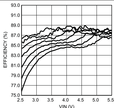
L = 22\text{ }\mu\text{H} 20 mA/String f_{SW} = 500\text{ kHz} Top To Bottom: 1×4, 1×5, 1×6, 1×7, 1×8, 1×9, 1×10 (LEDs)
