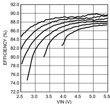
L = 22\text{ }\mu\text{H} 20 mA/String f_{SW} = 500\text{ kHz} Top To Bottom: 2×4, 2×5, 2×6, 2×7, 2×8, 2×9 (LEDs)
