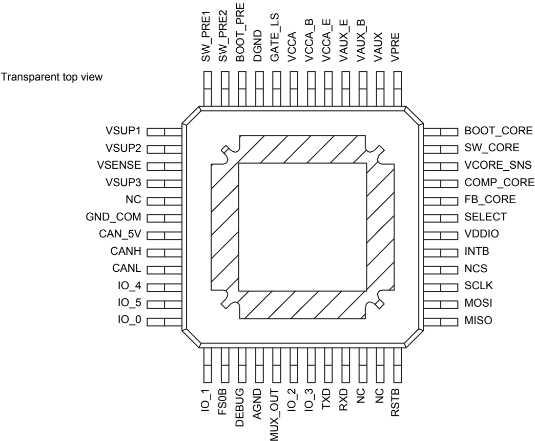
Figure 4. 33907_8 Pinout
