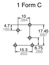
PC board pattern (Bottom view)
