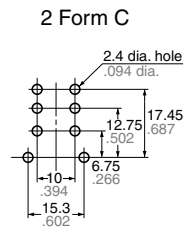
PC board pattern (Bottom view)
