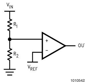
FIGURE 4. Threshold Detector
