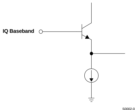
Figure 50. IVIN, QVIN, IREF, QREF Equivalent Circuit
