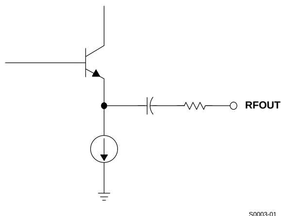
Figure 51. RFOUT Equivalent Circuit
