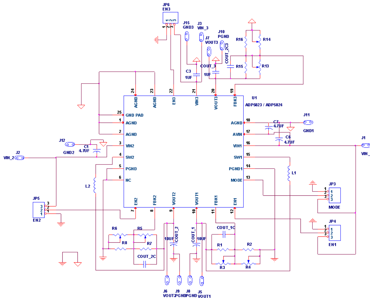
Figure 16. Evaluation Board Schematic of the ADP5023/ADP5024
