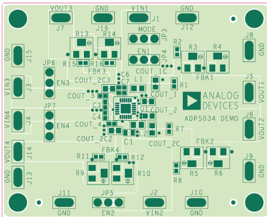
Figure 22. Top Layer, Recommended Layout for ADP5034/ADP5037
