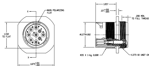
Part Dimensions for ATC-17-9-1939PN
