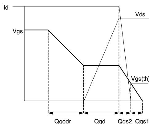
Fig 31b. Gate Charge Waveform
