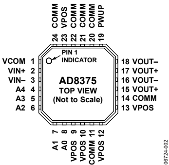
Figure 3. 24-Lead LFCSP
