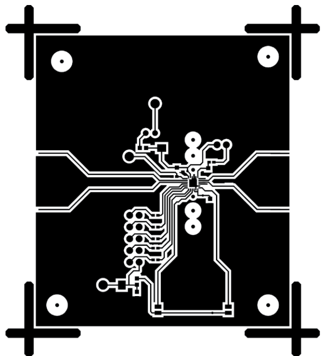
Figure 44. Differential-to-Differential Characterization Board Circuit Side Layout
