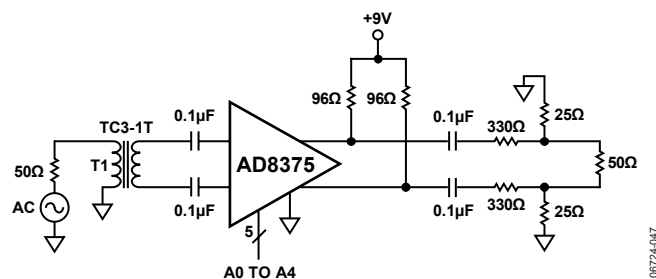
Figure 43. Test Circuit for Time Domain Measurements
