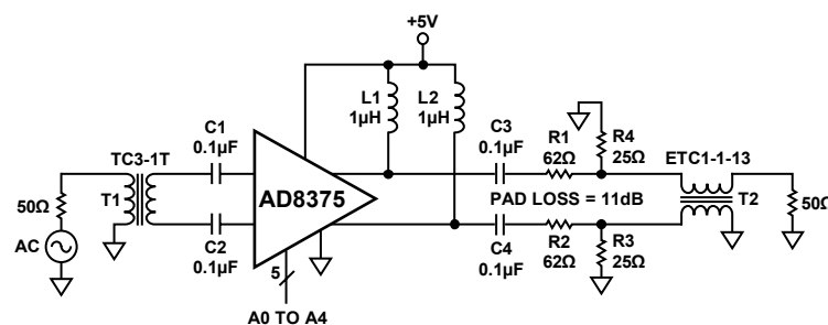
Figure 45. Test Circuit for Distortion, Gain, and Noise
