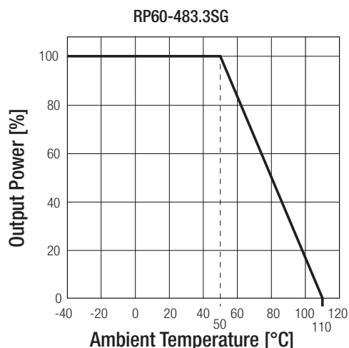
Derating Graph (11)
