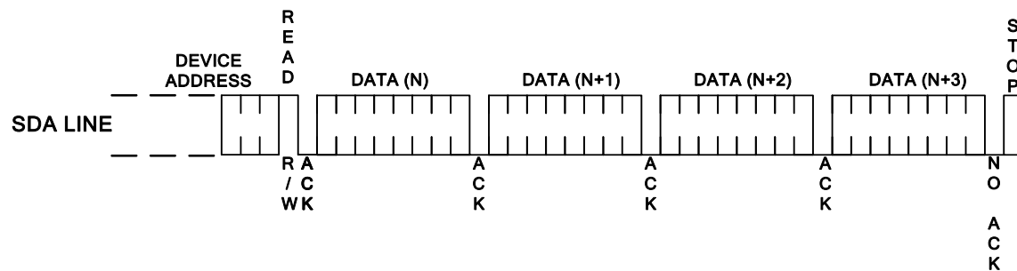
Figure 6: Sequential Read
