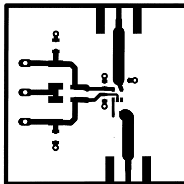
Top Silk
