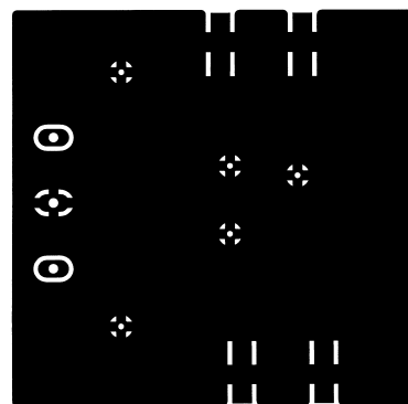
Bottom Copper
