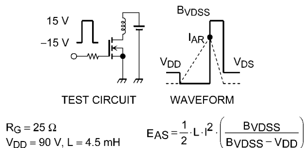
Fig. 8.16 Test Circuit/Waveform
