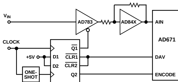
Figure 9. AD783 to AD671 Interface
