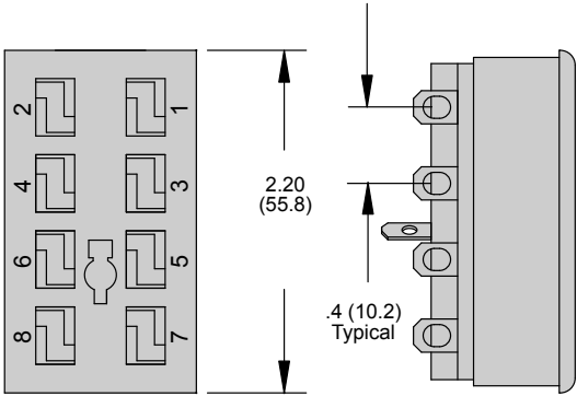
8 Pin Socket
