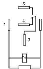
Terminal arrangement / Internal connections (BOTTOM VIEW)
