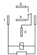
Terminal arrangement / Internal connections (BOTTOM VIEW)
