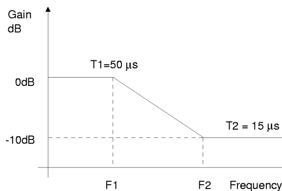
Figure 9. De-emphasis Curve
