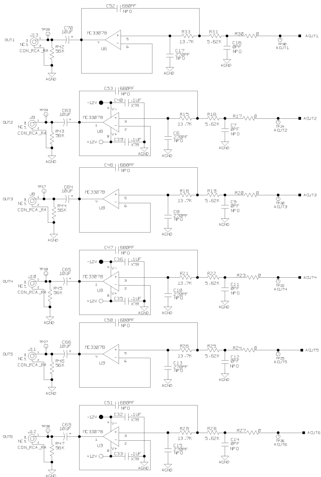
Figure 6. Analog Outputs
