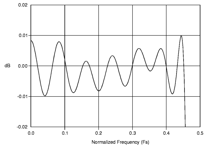
Figure 11. 20-bit ADC Passband Ripple
