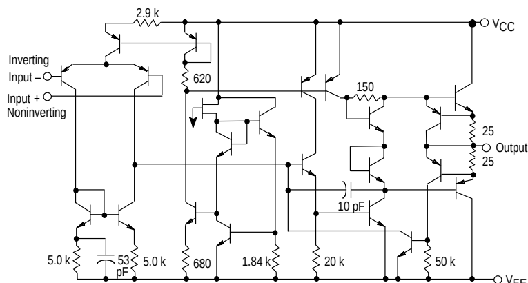
Representative Schematic Diagram (1/2 of Circuit Shown)
