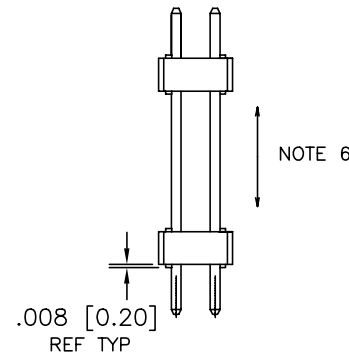
END VIEW
