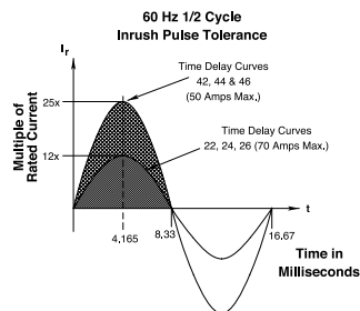
Pulse Tolerance Curves
