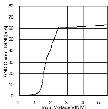
Fig.4 GND Current vs Input Voltage (BH25NB1WHFV)
