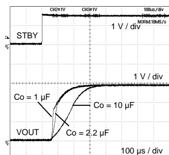
Fig.23 Output Voltage Rise Time (BH30NB1WHFV)
