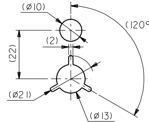
DETAIL "F"
