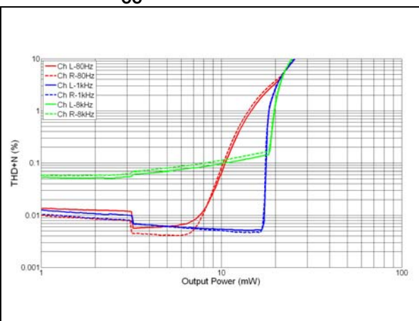
Figure 25. THD+N vs. output power - R_L = 32\ \Omega + I_{Pad} , in-phase, V_{CC} = 3.6\ V
