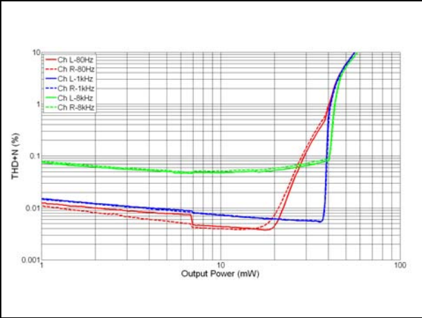
Figure 18. THD+N vs. output power - R_L = 32\ \Omega , out-of-phase, V_{CC} = 2.5\text{ V}
