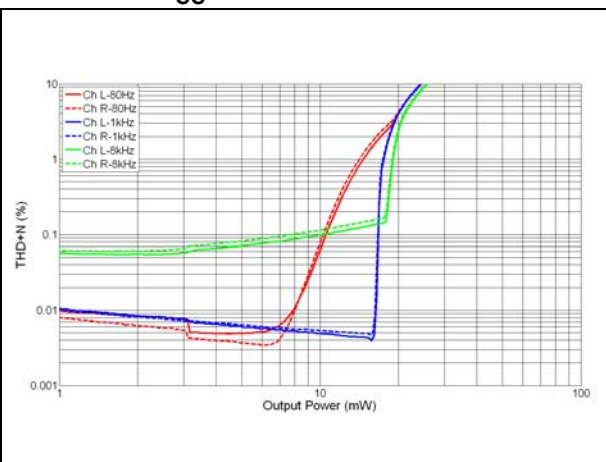
Figure 23. THD+N vs. output power - R_L = 32\ \Omega + I_{Pad} , in-phase, V_{CC} = 2.5\ V
